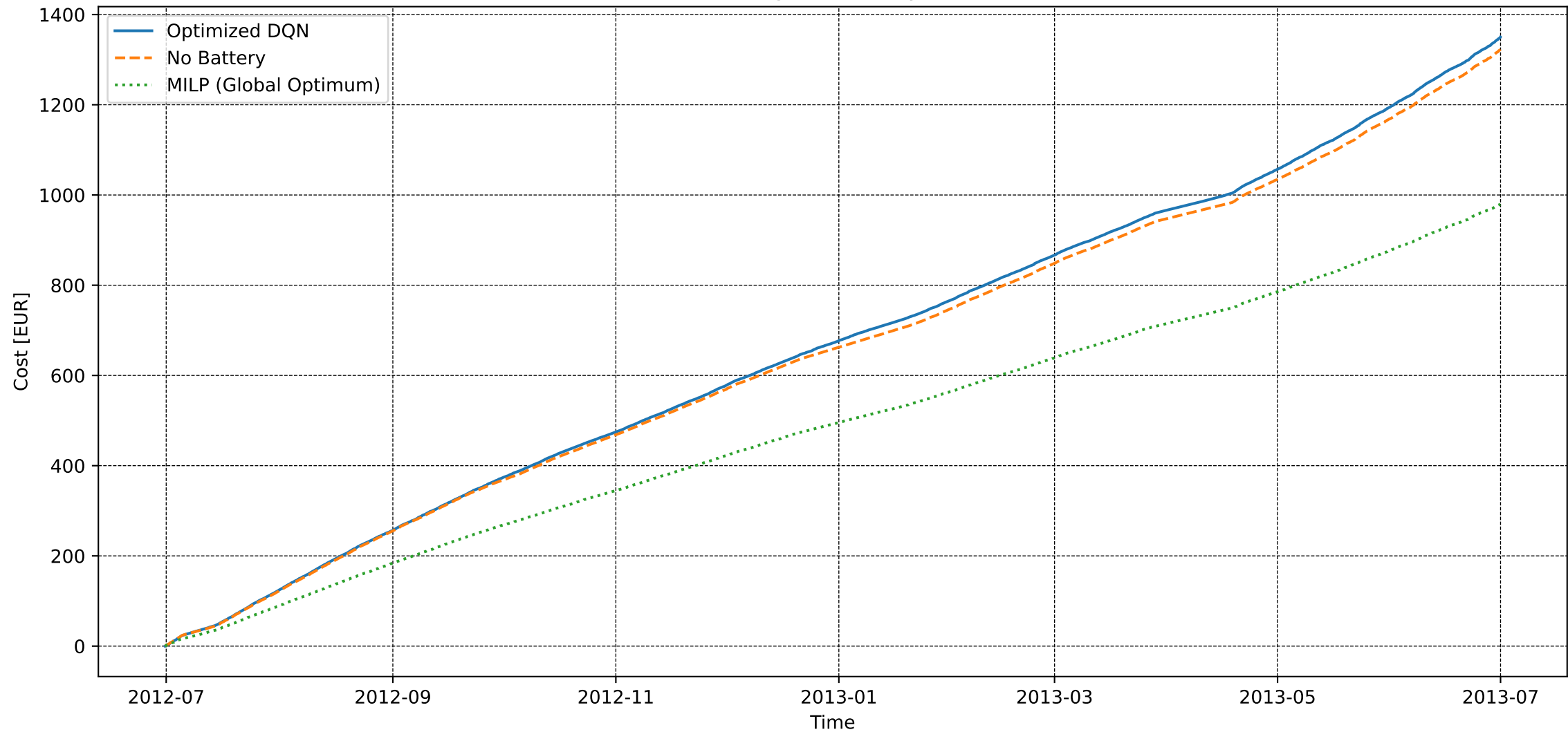
User 27 - Basic Training - Electricity Cost [DQN vs MILP]
